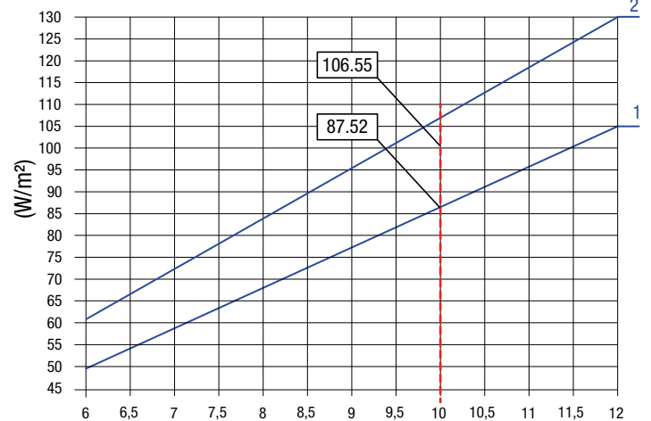
UNI EN 14037: summer thermal capacity (W/m 2 )
