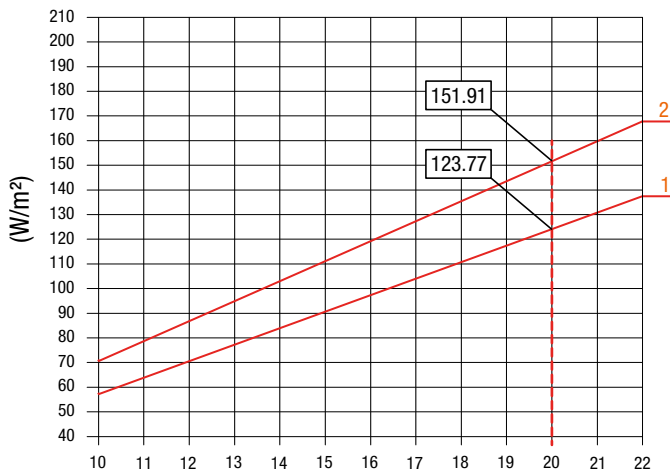
UNI EN 14240: winter thermal capacity (W/m 2 )
