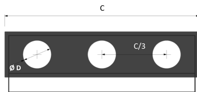
3 attacchi | 3 connectors
