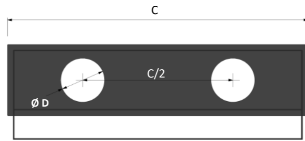
2 attacchi | 2 connectors
